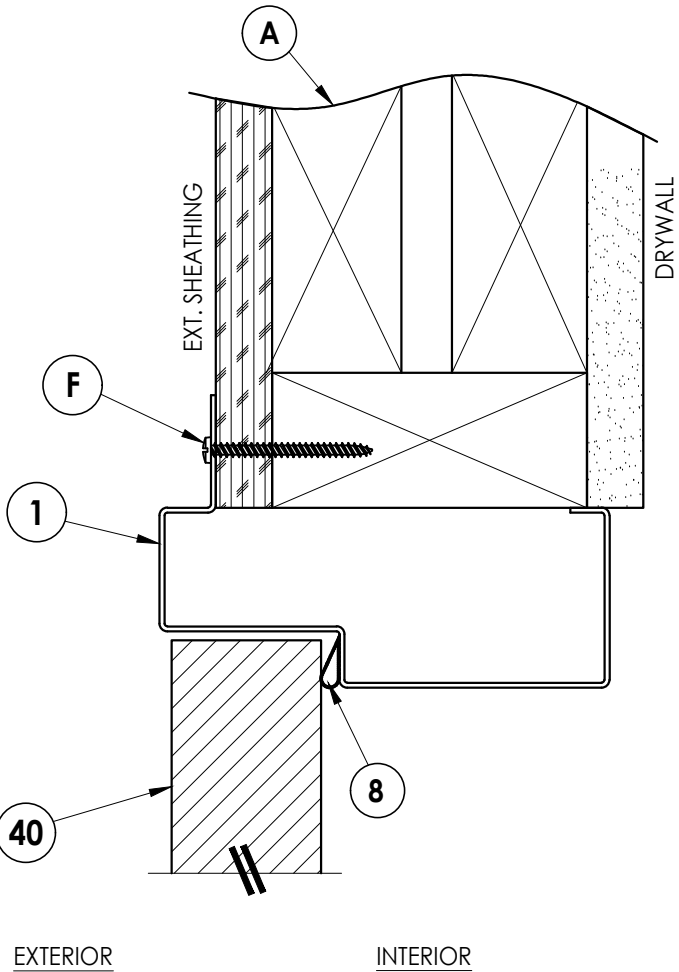
1 VERTICAL CROSS SECTION 4
